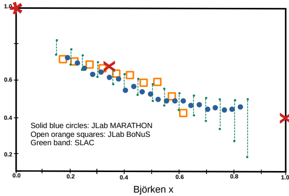
Fig. 9: Ratio of nucleon structure functions (Data from [19]); red crosses: values according to partial charges only, at x \approx 1/3 according to U+U+D and D+D+U units (2/3), at x=1 according to UD-units (2/5); Star at x=0 corresponds to an identical field distribution of E and B-fields in the nucleons, where the time average of E and B fields resulting in structures such as given in fig. 3, fig. 8 will be replaced by E(t) and B(t), both of identical strength for U and D.
