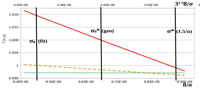
Fig. 5: \Gamma(+1/3, 8/\sigma) - green dots, lower x-scale / \Gamma(0, 3^{1.58}/\sigma) - orange dashes, upper x-scale / \Gamma(-1/3, 8/\sigma) - red continuous line, lower x-scale; black lines mark selected \sigma -values as discussed in the text; reference for \Gamma(0) is \alpha^{-1}/(8\pi) , for \Gamma(+1/3, x) \Rightarrow \Gamma(+1/3) for \Gamma(-1/3, x) \Rightarrow 36\pi^2 \Gamma(-1/3) 43 ;
