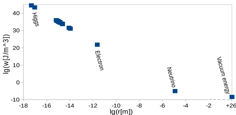
Fig. 4: Energy density, w , vs. length parameter, r (using Compton wavelength and \Lambda^{-0.5} ), for states described by this model 42 ;
